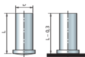
Goujons Lisses "AT"
